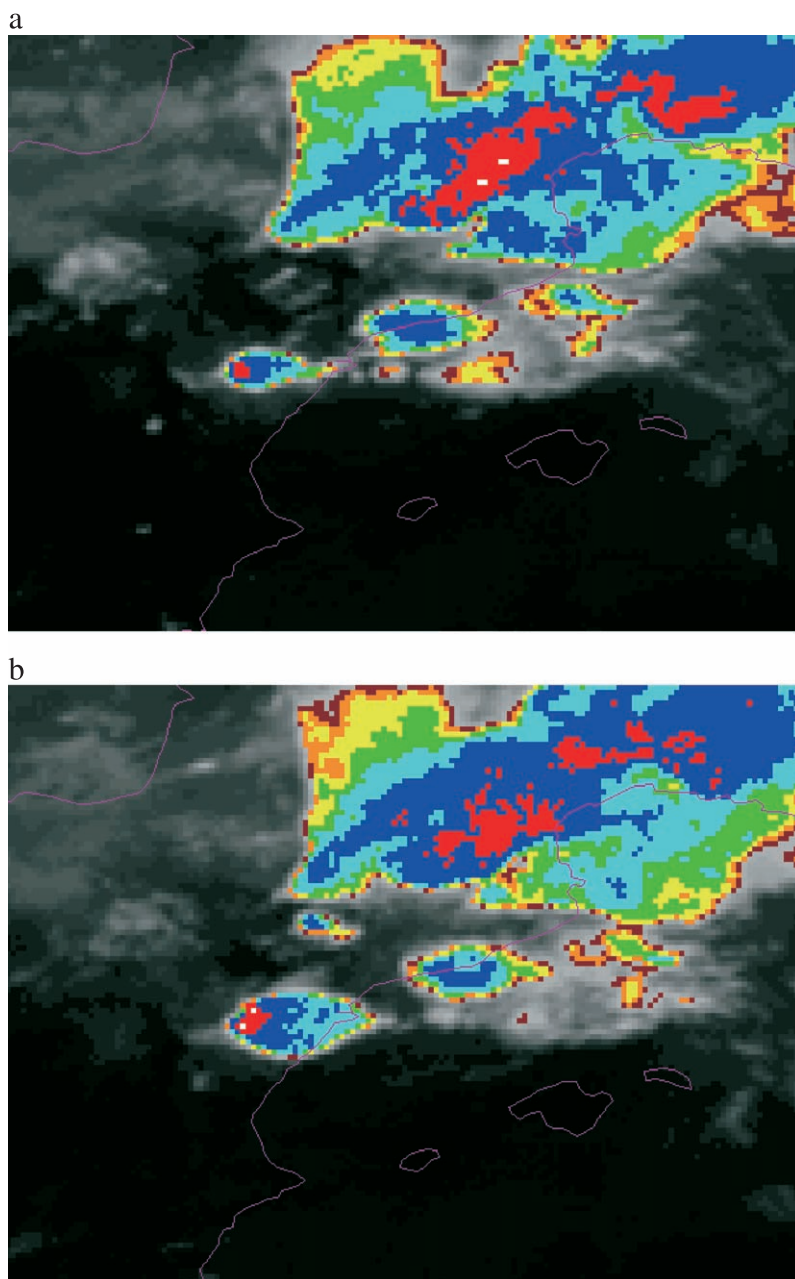
Fig. 5. Meteosat infrared images enhanced using a color palette for temperatures between -54 and -30 °C on 28 August at (a) 1800 UTC and (b) 1830 UTC.
