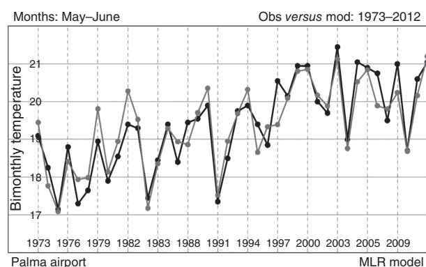
Figure 11. Observed (black line) versus modelled (grey line) local 2 m temperature at Palma airport, using a multi-linear-regression based on the main ten rotated PC obtained from the MJ 500-GH field in a large domain around Palma (Figure 10).
