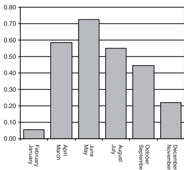
Figure 5. Bi-monthly temperature tendencies ( ^{\circ}\text{C } 10 \text{ years}^{-1} ). Palma airport, 1973–2012 homogenized series.
