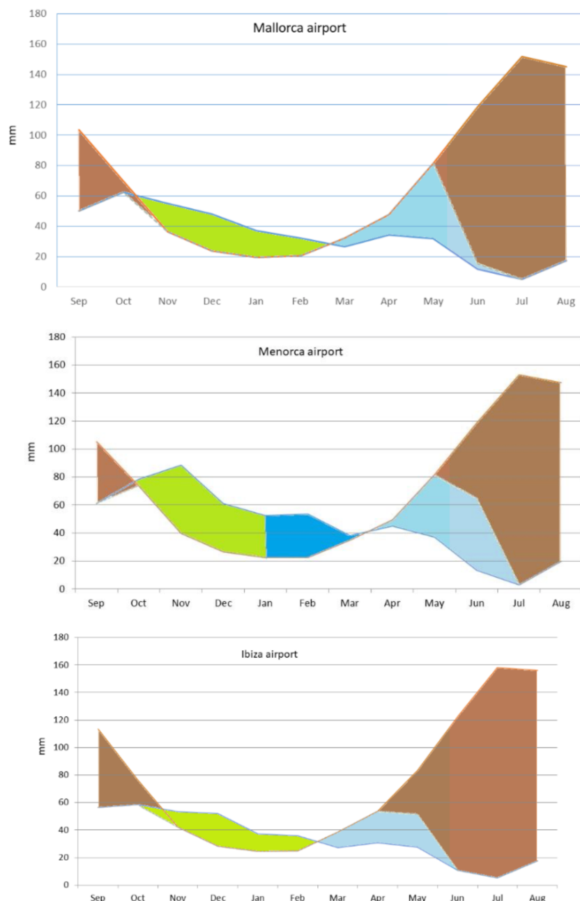
Figure 6. Climatic water balance (1981–2010) at the airports of Mallorca, Menorca and Ibiza (MaA, MeA and IbA in Fig. 1). Lines: blue is precipitation (mm); brown is potential evapotranspiration (mm); dashed green is evaporation (mm). Colored areas: green is the accumulation of water in the soil; cyan is the evaporation of water stored in the soil; blue is runoff; brown is the water deficit in the soil.
