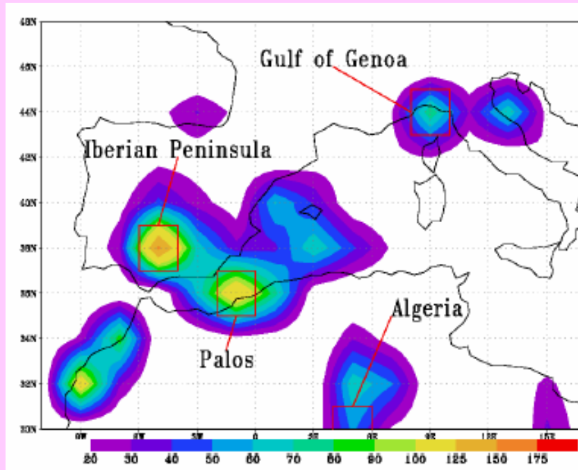
Shallow (1000-925 hPa)
