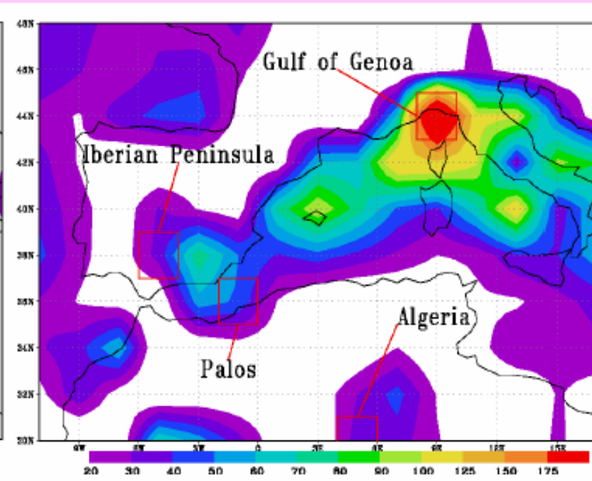
Deep (1000-300 hPa)
