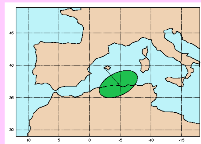
Balearic Islands
